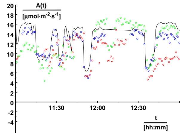
Photosynthese (simuliert - ; gemessen ● ● ● )
