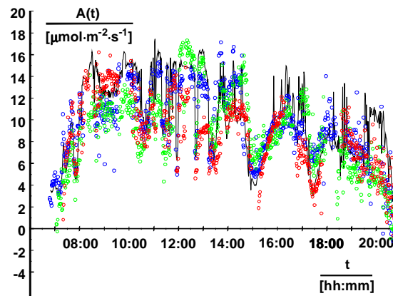
Photosynthese (simuliert - ; gemessen ● ● ● )
