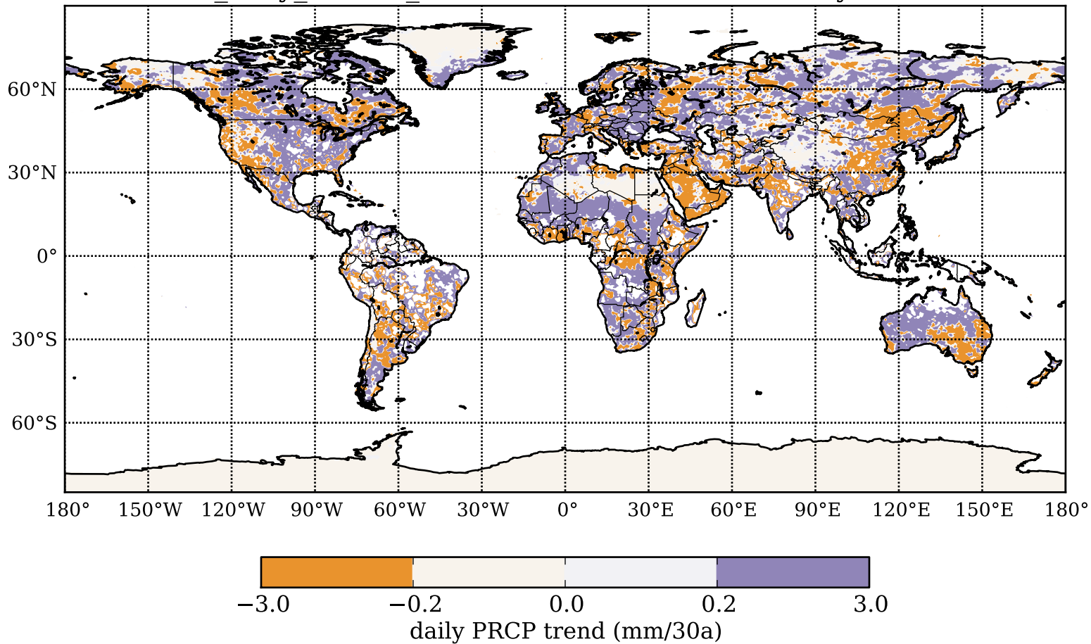
Rainf_daily_WFDEI_GPCC: 1979-2009, TREND, days > 20mm
