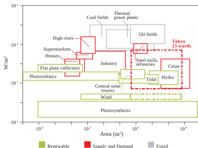
Figure 18.11 | Energy densities of energy supply from fossil (gray) and renewable sources (green) versus density of energy demand (red) for typical settings, in \text{W}/\text{m}^2 and \text{m}^2 area. Source: modified from Smil, 1991.
