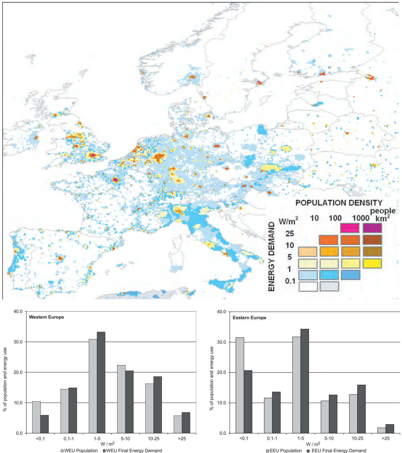
Figure 18.14 | Top: Spatially explicit energy demand densities in Europe (W/m²): Blue and white areas indicate where local renewables can satisfy low-density energy demand (<0.5–1 W/m²). Yellow, red and brown colors denote energy demand densities above 1, 5, 10, and 25 W/m² respectively.
