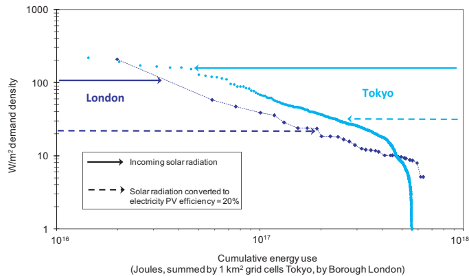
Figure 18.12 | Energy-demand densities ( \text{W/m}^2 ) for London (33 boroughs) and Tokyo (1 \text{km}^2 grid cells, 23 wards) versus cumulative energy use of these spatial entities (in Joules). For comparison the energy flux of incoming solar radiation ( \text{W/m}^2 ) and the electricity that could be generated (assuming photovoltaics (PVs) with a conversion efficiency of 20%) is also shown. Source: Dhakal et al., 2003; UKDECC, 2010.
