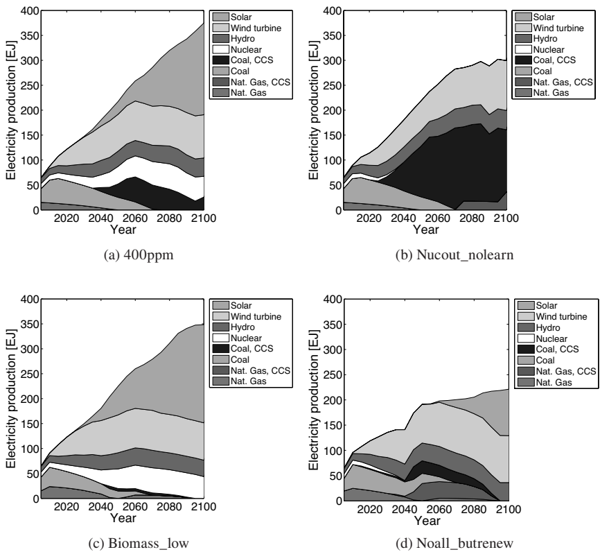
Figure 10. Global Electricity Production
