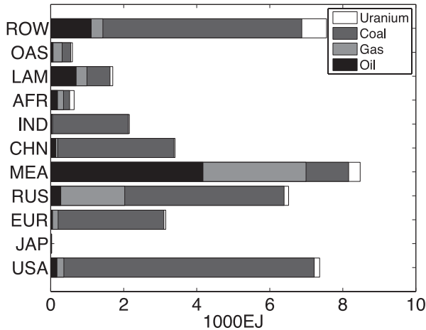
Figure 2. Reserve Endowments of Exhaustible Primary Energy Carriers
