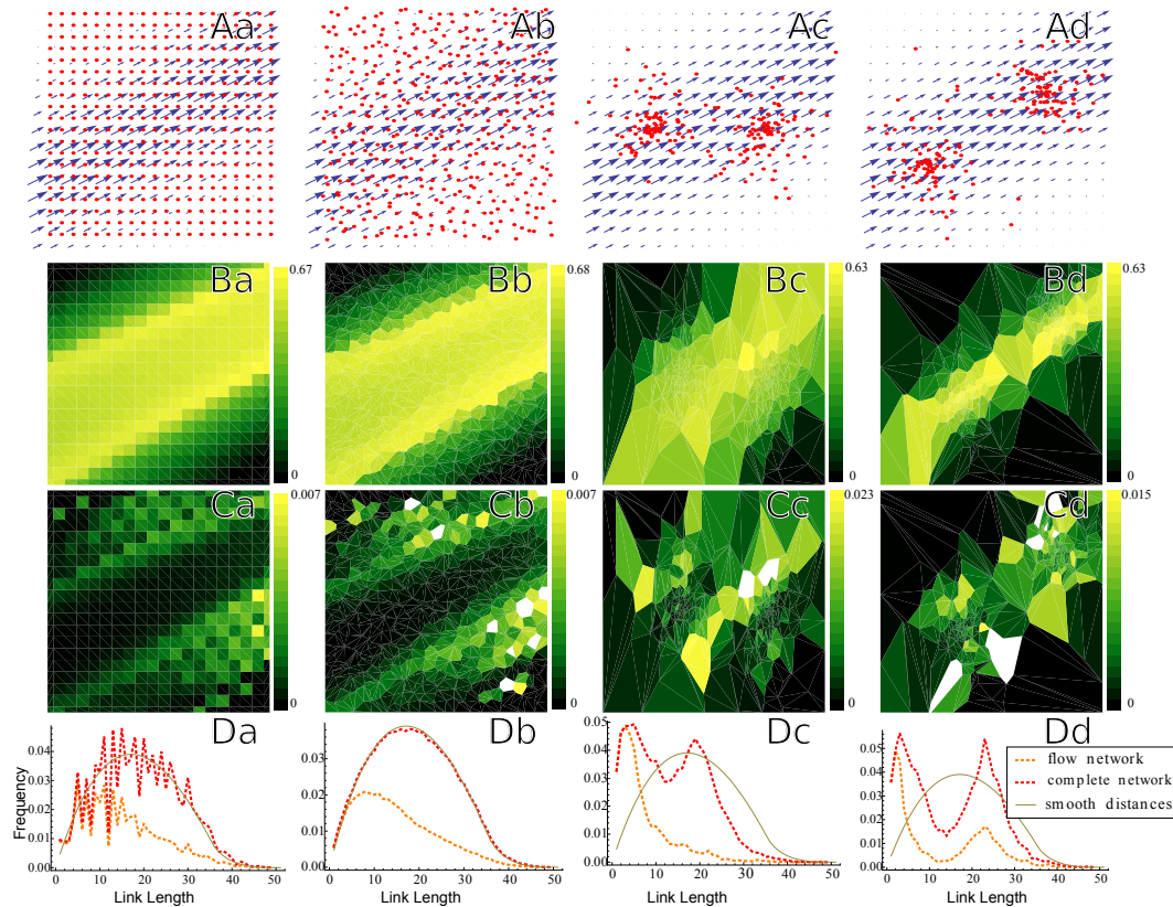
Figure 1. A diagonal flow is sampled with (Aa) a grid, (Ab) a jittered grid, (Ac) two clusters on opposite sides of the flow, and (Ad) two clusters inside the flow. The networks are constructed with a link density of 40 %. Row (B) shows the degree, row (C) the betweenness and row (D) the link length distribution.
