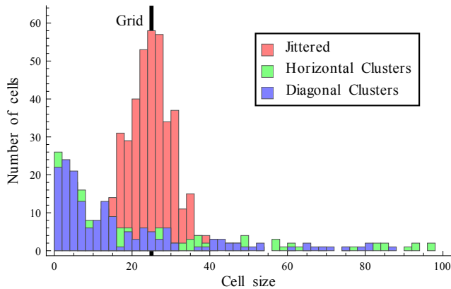
Figure 2. Tile size distribution for jittered and clustered sampling. The jittered sampling is peaked around the grid cell size, with clustered sampling results in many small and few very large tiles. Note that grid and jittered grid have twice as many nodes as the clustered sampling.
