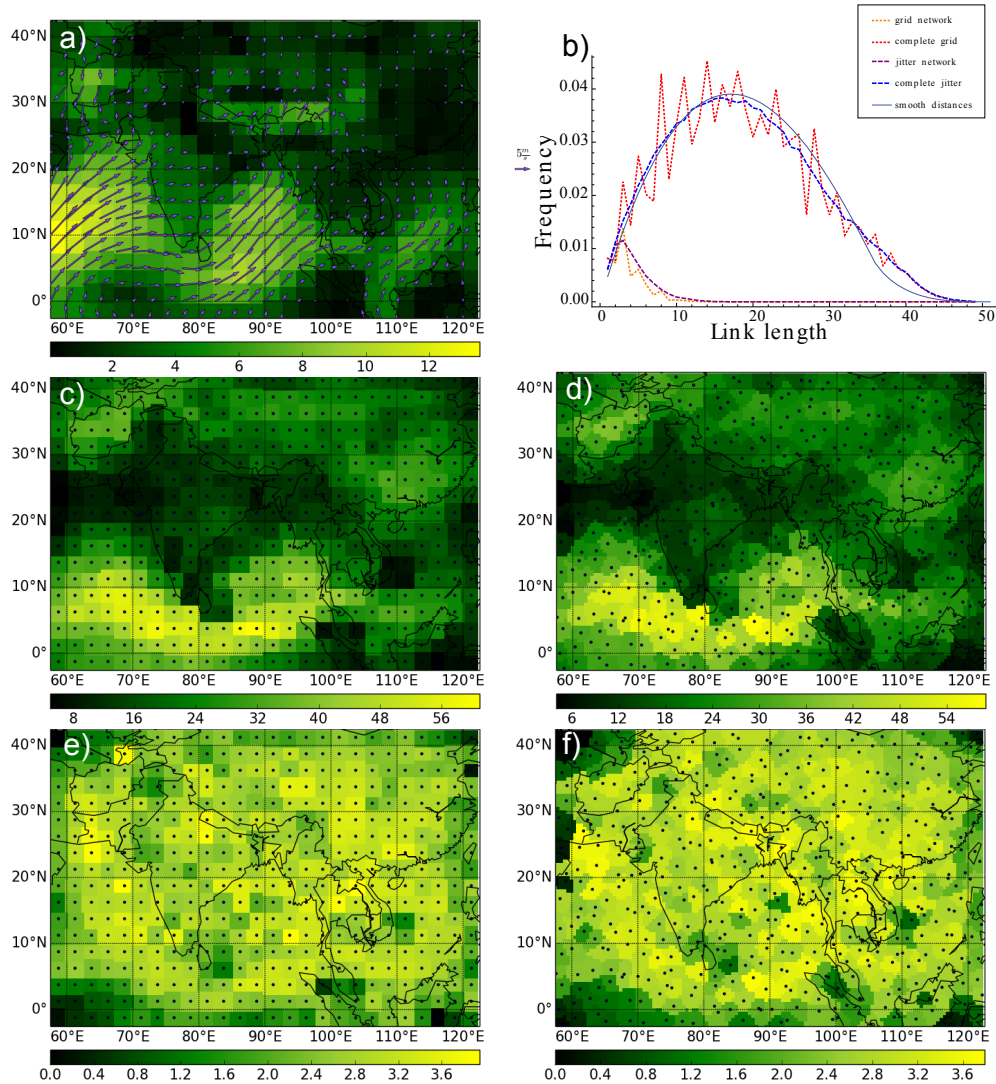
Figure 7. The correlation network of temperature data from NCEP/NCAR on a grid and a jittered grid. (a) Absolute mean wind velocity, (b) link length distributions, (c) degree of the grid network, (d) degree of the jittered network, (e) betweenness of the grid network, (f) betweenness of the jittered network.
