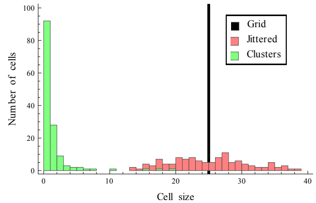
Figure 3. Tile size distribution for the three node distributions in START.
