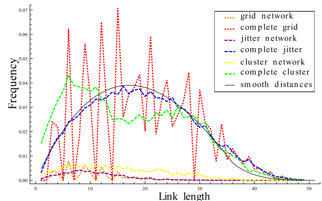
Figure 4. Link length distribution for the three node distributions in START.
