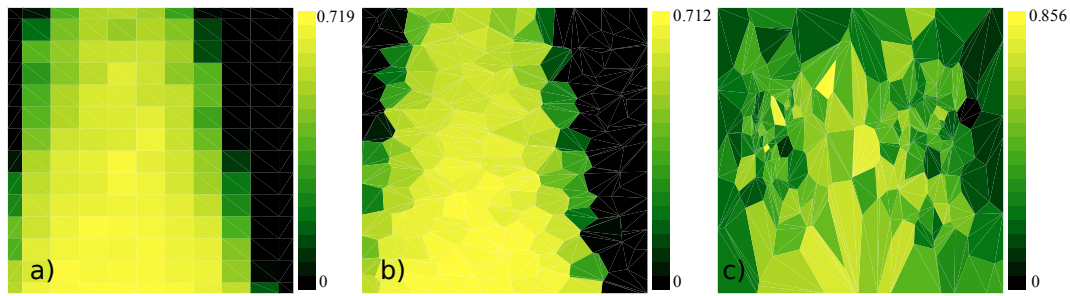
Figure 5. Degree of the network of the flow generated with START for grid (a), grid with jitter (b) and two clusters (c).
