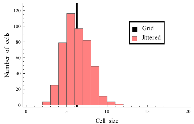
Figure 6. Tile size distribution for the jittered tile size distribution of the reanalysis data together with the grid line.
