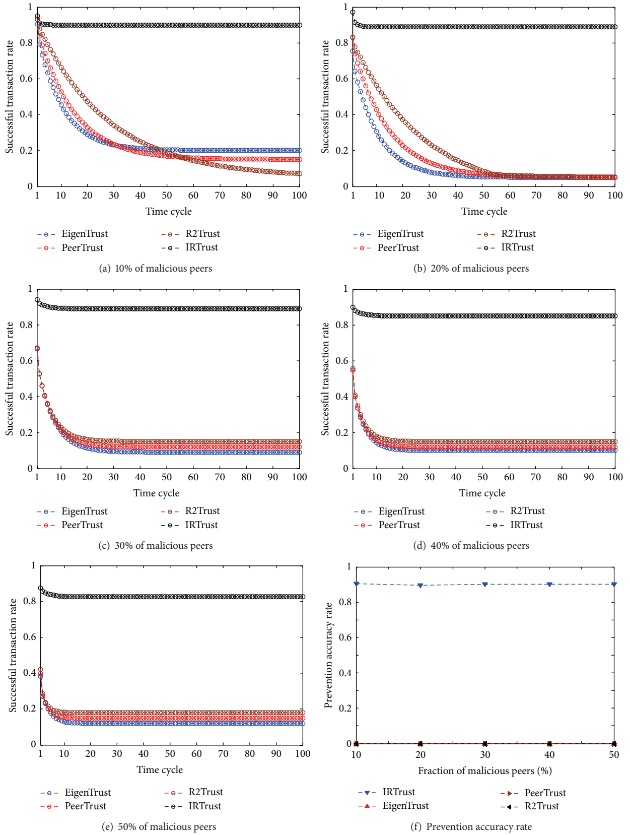
FIGURE 7: Performances of IRTrust, EigenTrust, PeerTrust, and R2Trust in sybil attack (color online).
