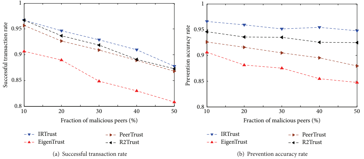
FIGURE 4: Performances of IRTrust, EigenTrust, PeerTrust, and R2Trust in simple attack (color online).
