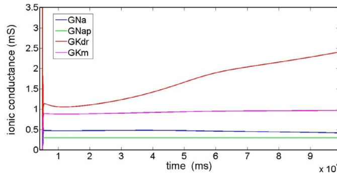
Fig. 8. Conductance variations during SD ( I_D = 1.8 \mu\text{A}/\text{cm}^2 ).
