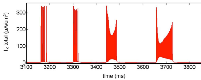
Fig. 3. The depression of K^+ currents over the time ( I_{K \text{ total}} = I_{Kdr} + I_{Km} + I_{KA} + I_{KL} ). The direct current used in this simulation was I_D = 1.5 \mu\text{A}/\text{cm}^2 .
