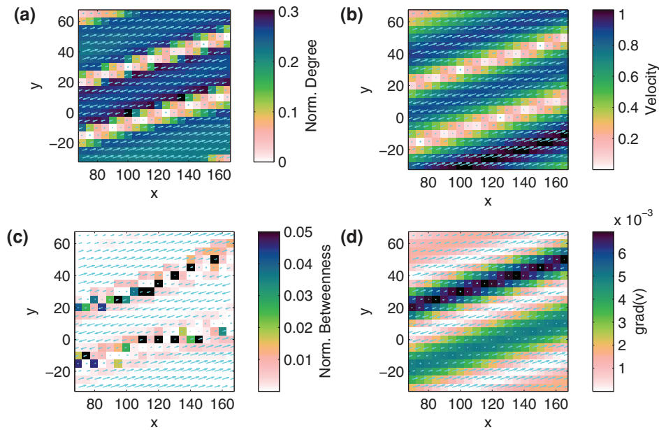
Figure 2 | Flow field and network measures for the counter-currents in Fig. (1a). (a) The normed degree, relates to (b) the absolute value of the flow's local velocity; (c) The maxima of the normed betweenness are co-located with (d) the maxima of the absolute value of the gradient gradient of the absolute current velocity. See equations (14) and (15) for definitions of the network measures.
