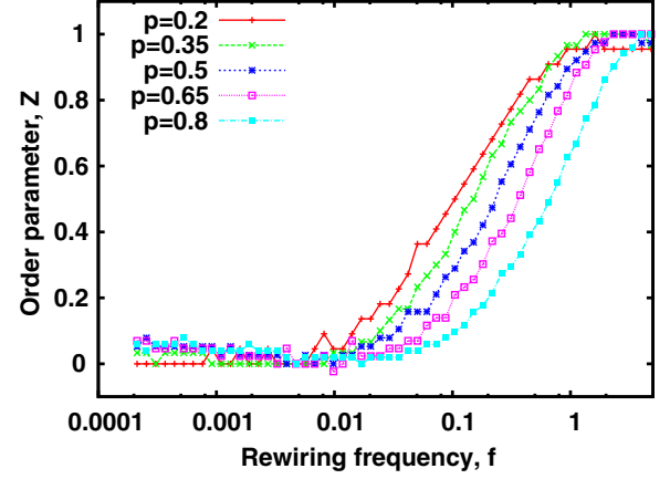
FIG. 7. (Color online) Order parameter Z as a function of rewiring frequency f . One can see that order parameter for low p values increases at lower values of rewiring frequencies.
