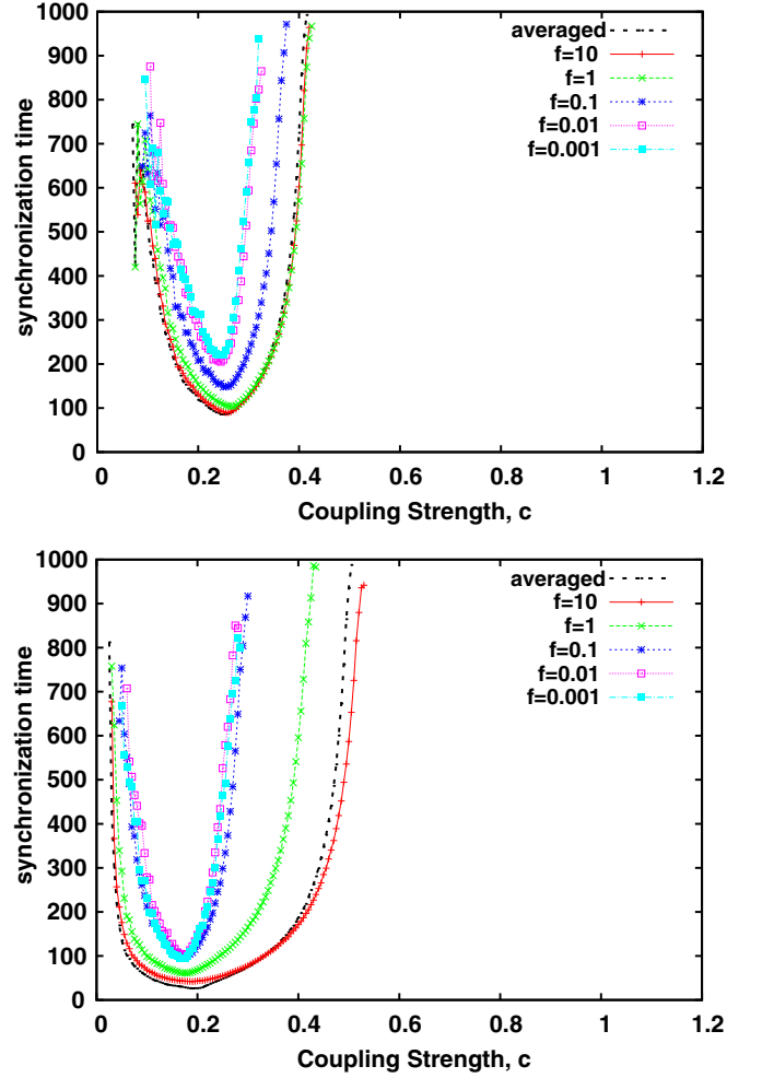
FIG. 3. (Color online) Time taken to reach the synchronized state for various coupling strengths, and rewiring frequencies at p = 0.2 (top) and p = 0.8 (bottom) for k = 4 . It can be seen that fast rewiring networks take much lower time to reach the synchronized state.
