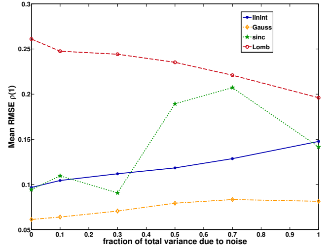
Fig. 10. Effect of the Signal-to-Noise ratio on the RMSE of the ACF for skewed ( sk = 2 ) inter-observation times. The share of the noise variance in the overall process variance increases from left to right (cf. Eq. 17).
