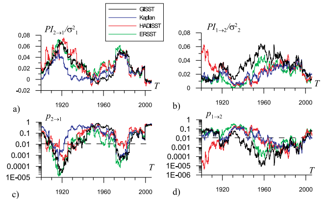
Figure 3. (a and c) Estimates of the ENSO-to-monsoon and (b and d) monsoon-to-ENSO influence in a moving window [T - W, T] versus the coordinate of window endpoint T ( W = 30 years). The dashed lines show Bonferroni corrected pointwise significance levels corresponding to the resulting significance level p = 0.05 (see text). Different colors mean the results for different Niño-3 indices.
