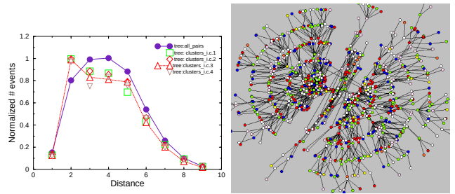
FIG. 6 (color online) Left: Distribution of the topological distances for a tree with 1000 nodes (bullets) and the distance inside the synchronized clusters (other symbols) for \sigma = 0.017 and different initial conditions. Right: visualization of the tree with five interconnected clusters of synchronized nodes marked by different colors. From Levnajic and Tadic (2007).
