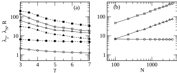
FIG. 11 Synchronizability of random SF networks. Plotted are eigenvalues \lambda_2 (circles) and \lambda_N (squares) and eigenratio R (triangles). (a) As functions of the exponent \gamma for network size N = 2^{10} ; open symbols for k_{\min} = 5 and filled symbols for k_{\min} = 10 . (b) As a functions of network size N at \gamma = 3 and k_{\min} = 10 . The results are averaged over 50 realizations.
