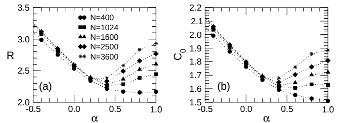
FIG. 24 Eigenratio R (a) and normalized cost C_0 (b) as a function of the parameter \alpha in Eq. (96), for random SF networks with \gamma = 3 and k_{\min} = 10 . From Motter et al. (2005c)
