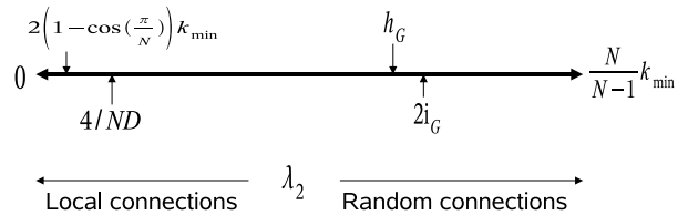
FIG. 16 A schematic plot of the bounds of \lambda_2 for networks with minimal degree k_{\min} .
