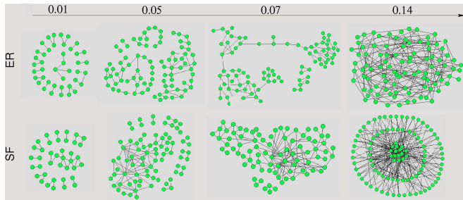
FIG. 3 (color online) Synchronized components for several values of \sigma for the two limiting cases of ER and SF networks. The figure clearly illustrates the differences in forming synchronization patterns for both types of networks: in the SF case links and nodes are incorporated together to the largest of the synchronized clusters, while for the ER network, what is added are links between nodes already belonging to such cluster. From Gómez-Gardeñes et al. (2007a).
