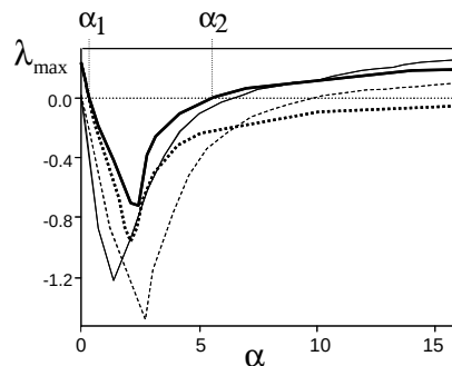
FIG. 8 Four master stability functions for coupled Rössler oscillators: chaotic (bold) and periodic (regular lines); with y coupling (dashed) and x coupling (solid lines). (The curves are scaled for clearer visualization). From Barahona and Pecora (2002).
