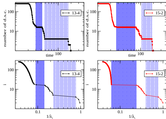
FIG. 4 (color online) Top: Number of disconnected synchronized components (d.s.c.) as a function of time. Bottom: Rank index versus the corresponding eigenvalue of the Laplacian matrix. Each column corresponds to a network with two hierarchical levels of communities. The difference lies in the relative weight of the two modular levels. From Arenas et al. (2006 b ).
