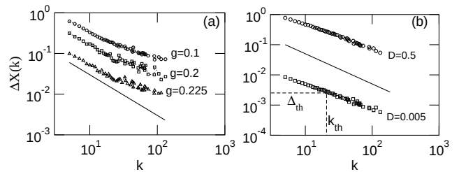
FIG. 28 The average values \Delta X(k) as a function of k in SF networks of Rössler oscillators outside the complete synchronization regime. (a) At various coupling strengths g = \sigma\langle k \rangle below the threshold for complete synchronization and (b) the synchronized state is perturbed by noise of different intensities D . Qualitatively, the same behavior is observed when the oscillators are nonidentical. From Zhou and Kurths (2006b).
