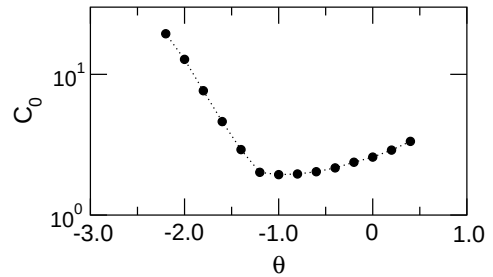
FIG. 18 Normalized cost C_0 as a function of \theta in Eq. (87) for random SF networks with \gamma = 3 , k_{\min} = 10 and N = 1024 . Modified after Motter et al. (2005a).
