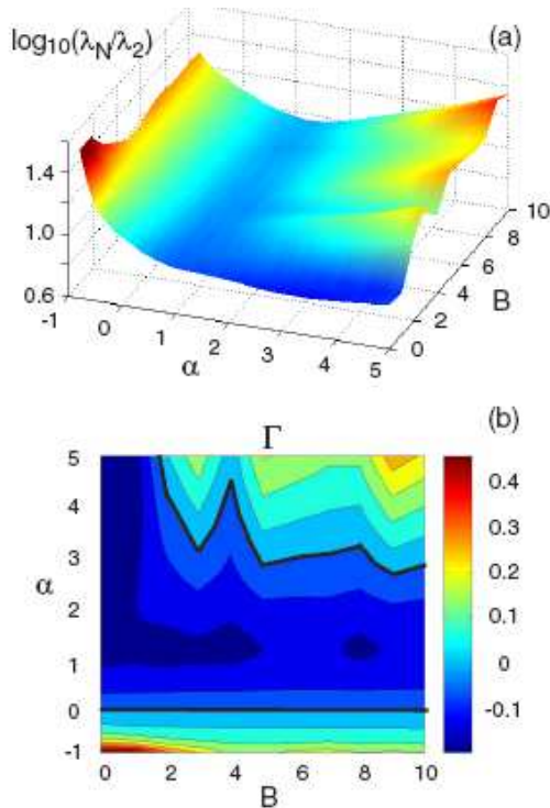
FIG. 23 (color online) (a) eigenratio \lambda_N/\lambda_2 (in logarithmic scale) for SF networks in the parameter space (\alpha, B) . (b) The relative synchronizability \Gamma = \log(\lambda_N/\lambda_2) - [\log(\lambda_N/\lambda_2)]_{\alpha=0} vs (\alpha, B) . In all cases m = 2 , and the graphs refer to averaging over 10 realizations of networks with N = 1000 . The domain with \Gamma < 0 is outlined by the black contours drawn on the figure. From Chavez et al. (2005).
