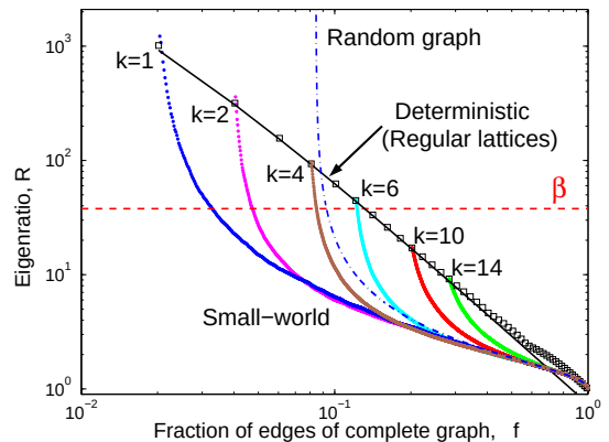
FIG. 9 (color online) Decay of the eigenratio R in a N = 100 lattice as a fraction f of the N(N-1)/2 possible edges are added following purely deterministic, semirandom, and purely random schemes. Networks become synchronizable below the dashed line ( \beta = \alpha_2/\alpha_1 , where \alpha_1 and \alpha_2 are from Fig. 8). The squares (numerical) and the solid line [analytic Eq. (63)] show the eigenratio decay of regular networks through the deterministic addition of short-range connections. The dot-dashed line corresponds to purely random graphs [Eq. (68)], which become almost surely disconnected and unsynchronizable at f \simeq 0.0843 . The semirandom approach (dots, shown for ranges k = 1, 2, 4, 6, 10, 14 ) is more efficient in producing synchronization when k < \ln N . From Barahona and Pecora (2002).
