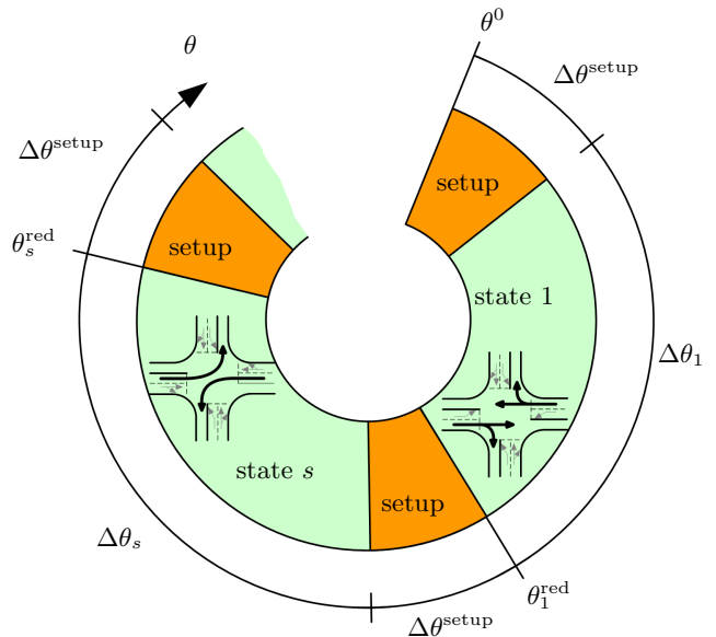
FIG. 34 (Color online) A single intersection adjusts the mapping of the phase-angle \theta to the switching states s locally. Within a complete cycle, each state s is sequentially activated for a period \Delta\theta_s , during which the corresponding non-conflicting traffic lights are set to green. While switching from one state to another, all traffic lights are set to red for a period of \Delta\theta^{\text{setup}} . The phase-angle, at which a new cycle starts, is denoted by \theta_0 . From Lämmer et al. (2006).
