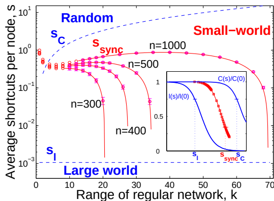
FIG. 12 (color online) Synchronizability thresholds S_{\text{sync}} (o) for graphs with N nodes ( N = 300, 400, 500, 1000 ) and range k \in [1, 70] , averaged over 1000 realizations. Solid lines are based on an analytical perturbation (Eqs. (66,67) valid in N^{1/3} < k < k_{\text{sync}}^0 ). For most parameters, S_{\text{sync}} lies within the SW region between the dashed lines (depicted for N = 1000 ), but it is distinct from its onset S_\ell . Inset: decay of the average distance \ell , clustering C , and eigenratio (squares) as shortcuts are added to a regular network of n = 500 and k = 20 . We define S_\ell and S_C as the points where \ell and C are 75% of the regular network value. From Barahona and Pecora (2002).
