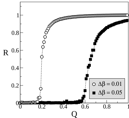
FIG. 29 Dependency of the order parameter R on the coupling strength Q , which is linearly proportional to the cell density. The two curves correspond to different values of the ratio between mRNA and protein lifetimes variance \Delta\beta . From García-Ojalvo et al. (2004).
