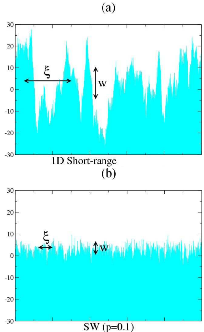
FIG. 33 (Color online) Virtual time horizon snapshots in the steady state for 10000 sites in one dimension. (a) For a regular network. The lateral correlation length \xi and width w are shown for illustration in the graph. (b) For the SW network with p = 0.1 , the heights are effectively decorrelated and both the correlation length and the width are reduced. From Guclu et al. (2006).
