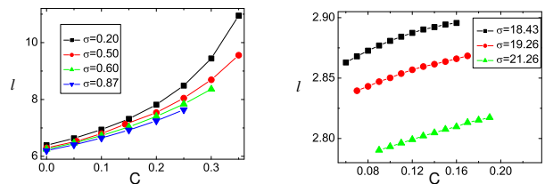
FIG. 14 (color online) The relationship between graph distance l and clustering coefficient C . Left: the original networks are the SW networks. Right: the original networks are the extensional BA networks. The different symbols are for different heterogeneity of degrees, measured by the standard deviation \sigma of the degree distribution. All the data are the average over 20 different realizations. From Zhao, Zhou, Wang, Yan, Yang and Bai (2006).
