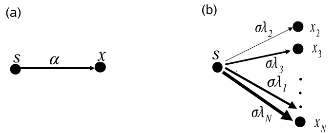
FIG. 7 Schematic plot of the eigenmode decomposition. (a) For 2 unidirectionally coupled nodes; (b) for a network of N coupled nodes.
