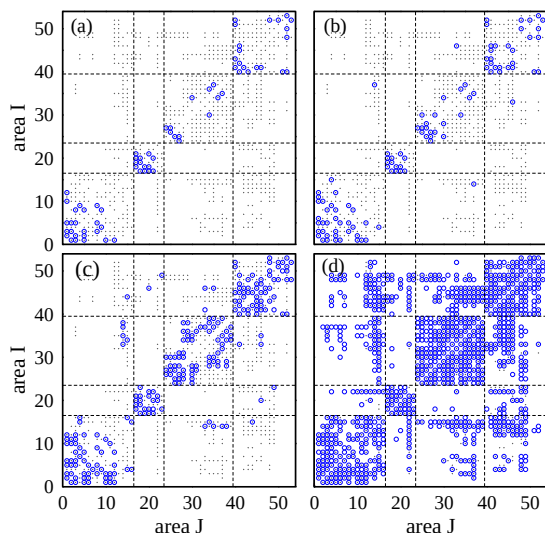
FIG. 31 (Color online) The functional networks (○) at various thresholds: R_{th} = 0.070 (a), R_{th} = 0.065 (b), R_{th} = 0.055 (c) and R_{th} = 0.019 (d). The small dots indicate the anatomical connections. From Zhou, Zemanová, Zamora, Hilgetag and Kurths (2006).
