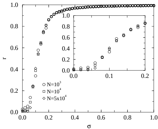
FIG. 2 Order parameter r (Eq. (4)) as a function of \sigma for several BA networks of different sizes. Finite size scaling analysis shows that the onset of synchronization takes place at a critical value \sigma_c = 0.05(1) . The inset is a zoom around \sigma_c . From Moreno and Pacheco (2004).
