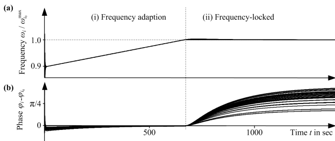
FIG. 35 Simulation results for a regular lattice road network, where the intersections are defined as oscillators with (a) a frequency \omega_i and (b) a phase \theta_i . From Lämmer et al. (2006).
