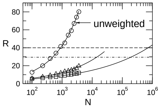
FIG. 26 The eigenratio R as a function of N averaged over 20 realizations of the networks. The solid lines are power-law fitting. The weighted networks are obtained by the adaptive process with the conditions: M = 5 , \gamma = 0.002 with \mathbf{H}(\mathbf{x}) = (x, 0, 0) for the Rössler oscillators ( \square ) and \mathbf{H}(\mathbf{x}) = (0, y, z) for the food-web model ( \triangle ). The networks are synchronizable if R < R_\alpha : Rössler oscillators, R_\alpha = 40 (dashed line), food-web model, R_\alpha = 29 (dashed-dotted line). From Zhou and Kurths (2006a)
