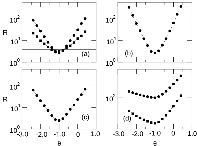
FIG. 17 Eigenratio R as function of \theta in Eq. (87): (a) random SF networks with \gamma = 3 ( \bullet ), \gamma = 5 ( \blacksquare ) and \gamma = \infty (solid line), for k_{\min} = 10 ; (b) random networks with expected SF sequence for \gamma = 3 and \tilde{k}_{\min} = 10 ; (c) growing SF networks for \gamma = 3 and m = 10 ; (d) SW networks with M = 256 ( \bullet ) and M = 512 ( \blacksquare ), for k = 1 . Each curve is the result of an average over 50 realizations for N = 1024 . Modified after Motter et al. (2005b).
