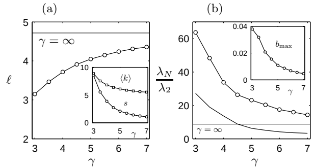
FIG. 13 Synchronizability of SF networks of size N = 1024 . The average network distance (a) and the eigenratio (b) for the random SF model with k_{\text{min}} = 5 . The inset of (a) shows the mean degree \langle k \rangle and the standard deviation s of the connectivity distribution. Inset of (b): the maximum normalized load b_{\text{max}} . The horizontal lines in (a) and (b) indicate the values of \ell and the eigenratio R for the \gamma = \infty case. The solid curve in (b) is the lower bound k_{\text{max}}/k_{\text{min}} in Eq. (76). The upper bounds of in Eq. (76) are above the limits, but follow the same trend. All quantities are averaged over 100 realizations. From Nishikawa et al. (2003).
