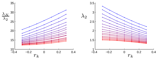
FIG. 15 (color online) Synchronizability of degree correlated SF networks of size N = 1000 , k_{\min} = 5 and \gamma = 2.5 . Left: Behavior of the eigenratio R . Right: behavior of the second lowest eigenvalue \lambda_2 . Both as functions of the correlation coefficient r_k defined in (Newman, 2002), for \gamma varying from 2 (blue line) to 5 (red line) in steps of 0.2. The results have been averaged over 100 different realizations. From di Bernardo et al. (2007).
