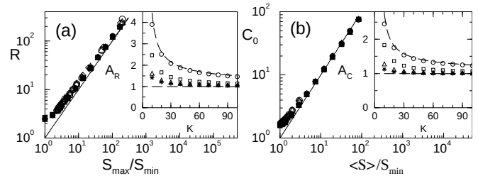
FIG. 20 (a) R as a function of S_{\max}/S_{\min} and (b) C_0 as a function of \langle S \rangle/S_{\min} , averaged over 50 realizations of the networks. Filled symbols: uniform distribution of S_i \in [S_{\min}, S_{\max}] . Open symbols: power-law distribution of S_i , P(S) \sim S^{-\Gamma} for 2.5 \leq \Gamma \leq 10 . Different symbols are for networks with different topologies: BA networks ( \circ ), growing SF network with aging exponent \alpha = -3 ( \square ), random SF network with \gamma = 3 ( \diamond ), and k -regular random networks ( \triangle ). The number of nodes is N = 2^{10} and the average degree is \langle k \rangle = 20 . Insets of (a) and (b): A_R and A_C as functions of \langle k \rangle for S_{\max}/S_{\min} = 1 ( \circ ), 2 ( \square ), 10 ( \triangle ), and 100 ( * ), obtained with uniform distribution of S_i in k -regular networks. The dashed lines are the bounds. Solid lines in (a) and (b): Eqs. (92) with A_R = A_C = 1 . From Zhou, Motter and Kurths (2006).
