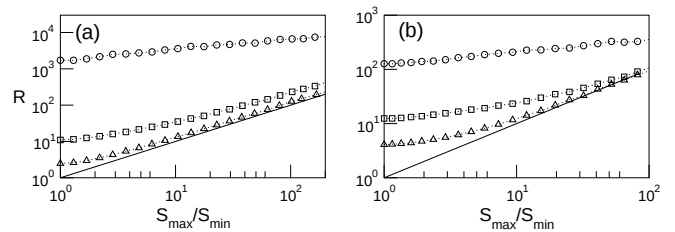
FIG. 22 (a) Eigenratio R as a function of S_{\max}/S_{\min} for BA growing networks with m = 1 ( \langle k \rangle = 2 ) ( \circ ), m = 2 ( \langle k \rangle = 4 ) ( \square ) and m = 10 ( \langle k \rangle = 20 ) ( \triangle ). (b) R for SW networks with \langle k \rangle = 20 and rewiring probability p = 0.01 ( \circ ), p = 0.1 ( \square ) and p = 0.3 ( \triangle ). Solid lines: Eqs. (92) with A_R = A_C = 1 .
