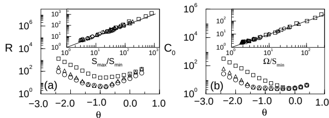
FIG. 21 (a) Eigenratio R and (b) cost C_0 as functions of \theta for BA networks ( \circ ), growing SF networks with aging exponent \alpha = -3 ( \square ) and random SF networks with \gamma = 3 ( \triangle ). Each symbol is an average over 50 realizations of the networks with \langle k \rangle = 20 and N = 2^{10} . Inset of (a): the same data for R as a function of S_{\max}/S_{\min} . Inset of (b): the same data for C_0 as a function of \langle S \rangle/S_{\min} . Solid lines: Eqs. (92) with A_R = A_C = 1 . From Zhou, Motter and Kurths (2006).
