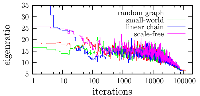
FIG. 27 (color online) Eigenvalue ratio R as a function of the number of algorithmic iterations. Starting from different initial conditions, with N = 50 , and \langle k \rangle = 4 , the algorithm converges to entangled networks with very similar values of R . From Donetti et al. (2005).
