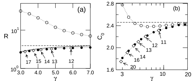
FIG. 19 Eigenratio R (a) and normalized cost C_0 (b) as a function of \gamma for random SF networks with \theta = 0 ( \circ ) and \theta = -1 ( \bullet ) and for random homogeneous networks with the same average degree \langle k \rangle ( \diamond ). The other parameters are k_{\min} = 10 and N = 1024 . The dashed line corresponds to \gamma = \infty ( \langle k \rangle = 10 ). The solid line in (a) is the approximation given by Eq. 91. Modified from Motter et al. (2005b).
