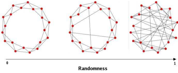
FIG. 1 Small-world network construction from a regular lattice by rewiring links with a certain probability (randomness), as proposed by Watts and Strogatz (1998)
