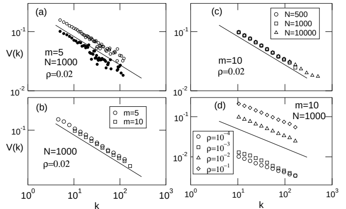
FIG. 25 The average input weight V(k) of nodes with degree k as a function of k for the Rössler oscillators ( \circ ) and the food-web model ( \bullet ) (a) and its dependence on various parameters: m (b), N (c) and \rho (d). Results in (b-d) are averaged over 10 realizations of the networks with random initial conditions. For clarity, only the results for the Rössler oscillators are shown in (b-d) and are logarithmically binned. The solid lines in (a-d) have a slope -0.48 . From Zhou and Kurths (2006a).
