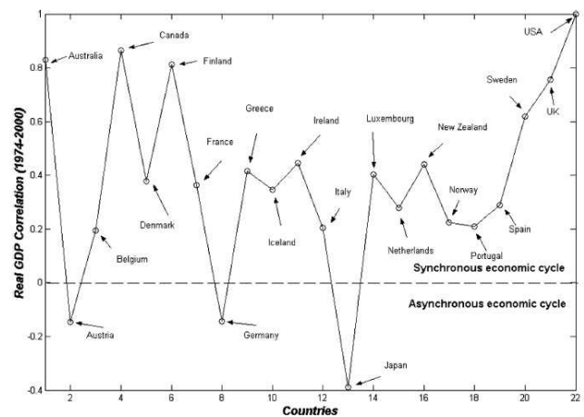
FIG. 36 Twenty-two developed countries' economic cycles synchronization phenomena. The positive real GDP correlation means synchronous economic cycles with the US. From Li et al. (2003).
