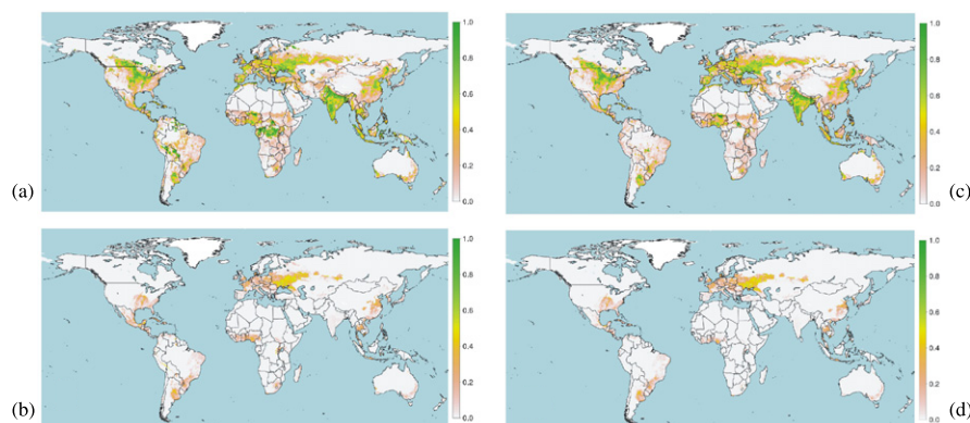
Figure 4. (a) Cell-specific share of total crop land and (b) share of bioenergy cropland in total cropland for the scenario with bioenergy (M) as well as (c) cell-specific share of total crop land and (d) share of bioenergy cropland in total cropland for the scenario with bioenergy and avoided deforestation (M_FC) (right column) in 2095.
