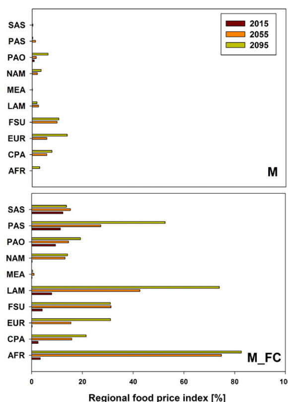
Figure 6. Regional food price index, i.e. the average of all cropping and livestock activities weighted with their share in total demand. The food price index describes relative changes to the reference scenario (no bioenergy demand for climate change mitigation and all suitable land available for cropland expansion) for each year.
