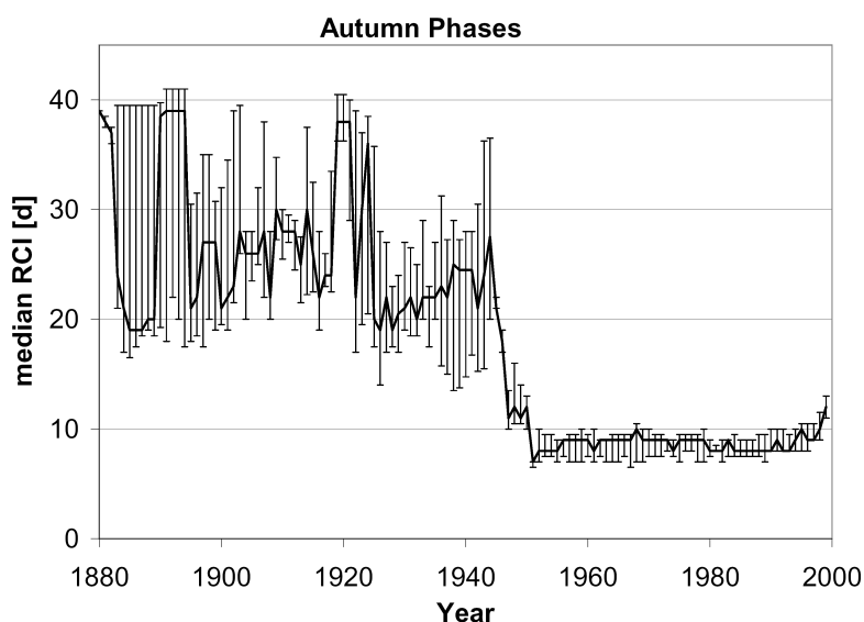
Figure 4-5. Median of the RCIs for the combined time series of Tab. 4-1 with 5% and 95% quantiles as error bars. Autumn phases (LC).
