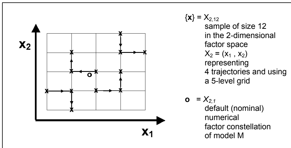
Fig. 4.2 Sample for a global sensitivity analysis The arrows indicate the sequence how sampling points were generated for each trajectory.
