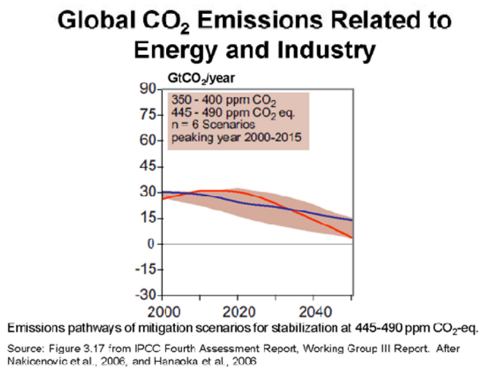
Figure 2 - Emission pathways for the lowest category assessed by IPCC AR4. Slide adapted from Figure 3.17 in IPCC AR4 WGIII 16 , as presented by the US (Jonathan Pershing) at the AWG-LCA workshop, 1st April 2009, Bonn, Germany. The blue line implies modest reduction rates, but assumes a peaking date of global emissions already in the past. The red lines peak global emissions before 2020, and implies higher reduction rates thereafter.
