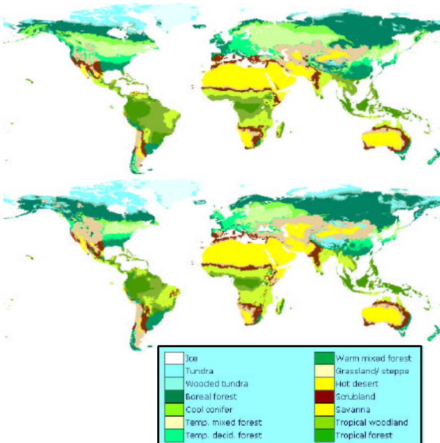
Natural vegetation patterns in 2100 for the two extremes in the scenario experiments: A1B_fastmigration (top) and A1B_nonegfb (bottom).
