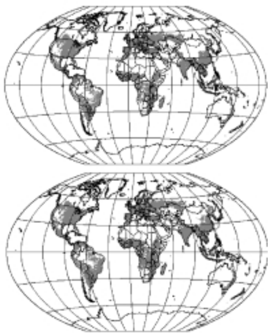
Fig. 5. Agricultural land in 2050 for the two extremes in the scenario experiments (A1B_constclim and A1B_nonegfb).
