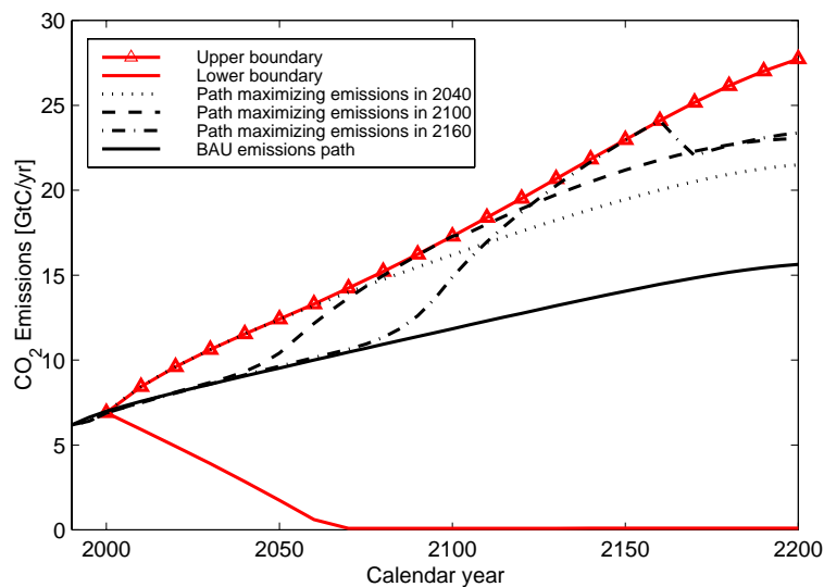
Figure 1. Emissions corridors — being the area between upper and lower boundaries — for standard parameter settings (see Table I). As an illustration of its internal structure, we show paths which maximize acceptable CO 2 emissions in 2040, 2100, and 2160. For comparison, we also display the reference (business-as-usual) emissions path which is the ‘no controls baseline’ obtained by applying the DICE model without climatic and welfare loss constraints.
