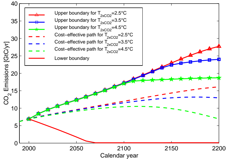
Figure 2. Emissions corridors for different values of climate sensitivity T_{2\times\text{CO}_2} (with all other model parameters and guard-rails held at their standard values). The lower corridor boundary is the same for all values of T_{2\times\text{CO}_2} , as this is solely determined by the maximum emissions reduction rate.
