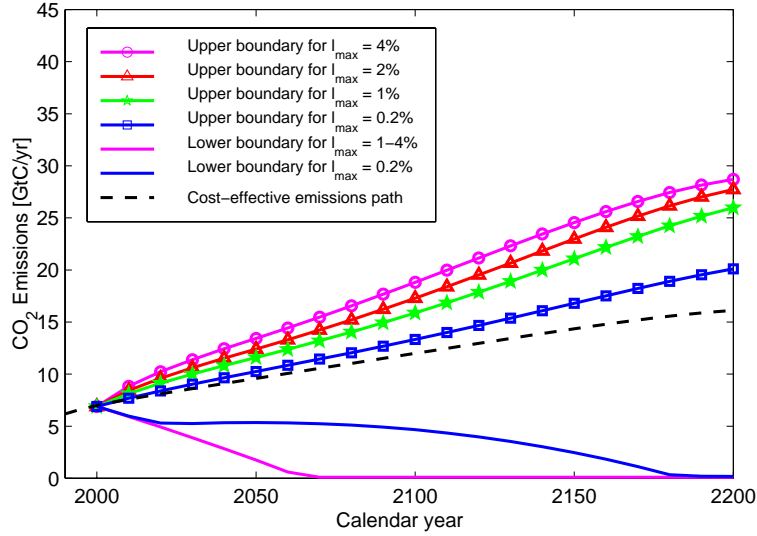
Figure 4. Emissions corridors for different values of the maximum admissible welfare loss l_{\max} (with all other model parameters guard-rails held at their standard values).
