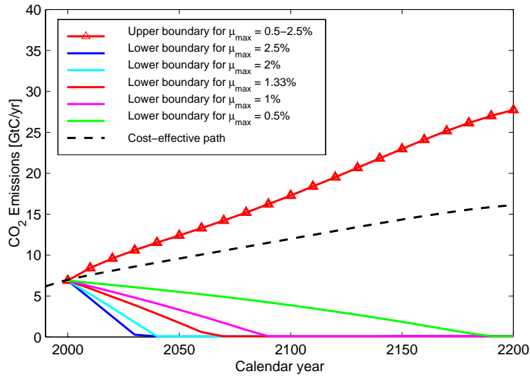
Figure 5. Emissions corridors for different values of the maximum emissions reduction rate \mu_{\max} (with all other model parameters and guard-rails held at their standard values).
