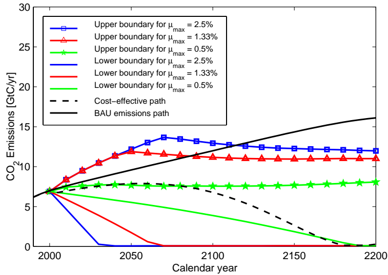
Figure 7. Emissions corridors for different values of the maximum emissions reduction rate \dot{\mu}_{\max} under worst-case conditions T_{2 \times \text{CO}_2} = 4.5^\circ \text{C} and h_2 = 0.05 \text{ Sv}^\circ \text{C}^{-1} (with all other model parameters and guard-rails are held at their standard values).
