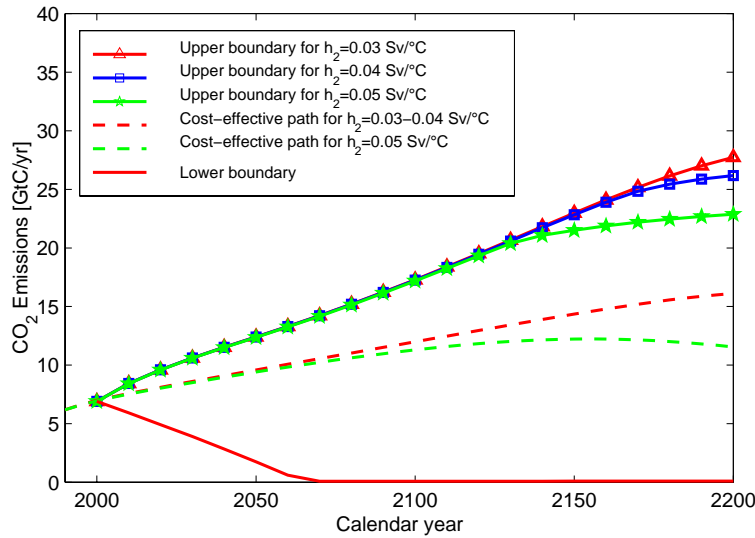
Figure 3. Emissions corridors for different values of the North Atlantic hydrological sensitivity h_2 (with all other model parameters and guard-rails held at their standard values). The lower corridor boundary is the same for all values of h_2 , as it is solely determined by the maximum emissions reduction rate.
