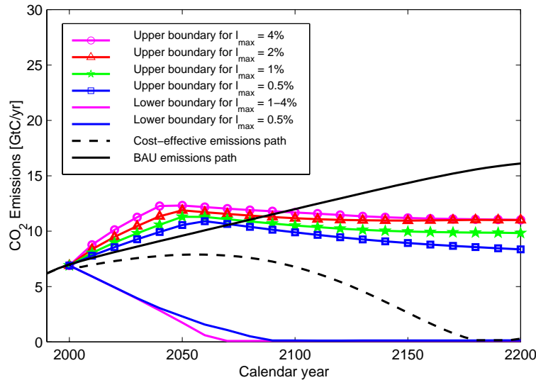
Figure 6. Least-cost emissions paths and emissions corridors for different values of the maximum admissible welfare loss l_{\max} under worst-case conditions T_{2\times\text{CO}_2} = 4.5^\circ\text{C} and h_2 = 0.05 \text{ Sv}^\circ\text{C}^{-1} (with all other model parameters and guard-rails are held at their standard values).
