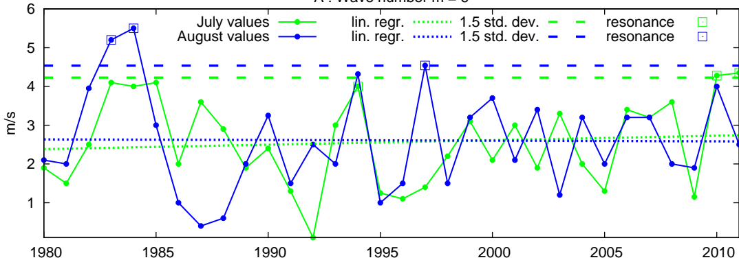
B : Wave number m = 7
