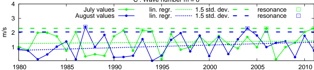
C : Wave number m = 8
