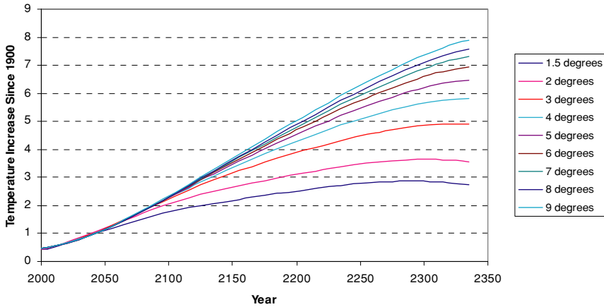
Fig. 1 Global mean temperature trajectories for the DICE-99 baseline emissions scenario determined for alternative climate sensitivities from 1.5–9 K and associated calibrations of the heat capacity of the atmosphere and the upper ocean layer (reprinted from Yohe et al. 2004, Figure S1)
