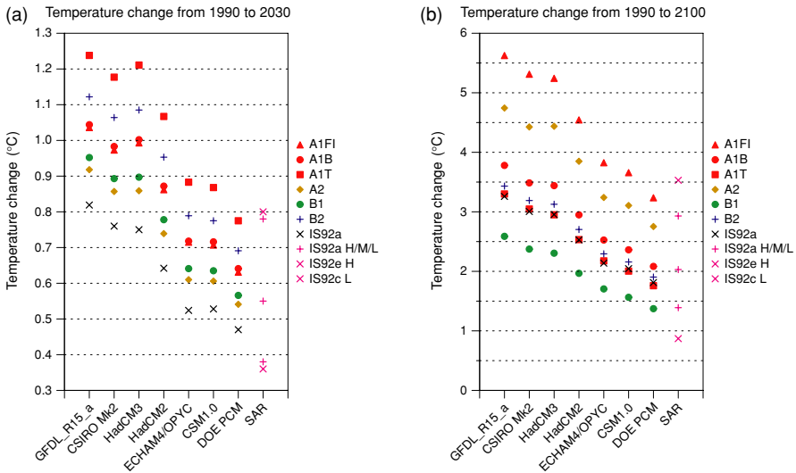
Fig. 2 Global mean temperature projections determined by the simple climate model MAGICC tuned to several GCMs from 1990 to 2030 (left plate) and 2100 (right plate) for the six illustrative SRES emissions scenarios (reprinted from Cubasch et al. 2001, Figure 9.15)
