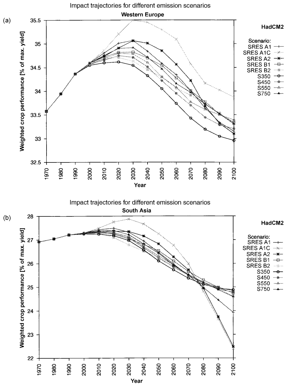
Figure 2. Weighted crop performance indices for (a) Western Europe and (b) South Asia. Note the different scales used in the two panels due to the differing ranges depicted.
