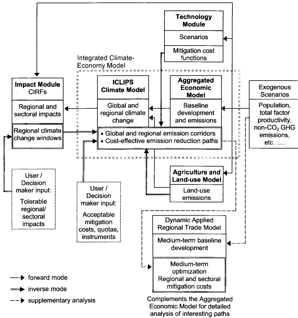
Figure 1. The structure and modes of application of the ICLIPS Integrated Assessment Framework. CIRFs = Climate Impact Response Functions.
