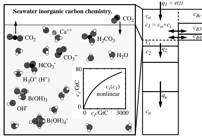
Figure 1. ICLIPS carbon-cycle model. ICLIPS CO 2 module: To the right, the cascade of oceanic layers, the uppermost of which represents the composite atmosphere-mixed layer, coupled to three terrestrial reservoirs. To the left, a zoom into the composite layer, for illustration of the nonlinear partitioning of the composite layer's carbon c_1 into its atmospheric and mixed-layer subsystems. c_a denotes the anthropogenic carbon in the atmosphere (in GtC), c_s the carbon perturbation in the oceanic mixed layer, and c_j the anthropogenic carbon in the j^{\text{th}} oceanic layer. The model includes an explicit treatment of the nonlinear sea water inorganic carbon chemistry resulting in a decreasing solubility of additional CO 2 in sea water as the background concentrations rise. The resulting nonlinear relationship between anthropogenic carbon c_s in the oceanic mixed layer and anthropogenic carbon c_1 in the composite layer (comprising the oceanic-mixed layer and the atmosphere) is depicted explicitly. e(t) denotes anthropogenic carbon emissions, q_j represents the carbon flux from layer j - 1 into layer j , c_{B_i} is the anthropogenic carbon in land biosphere reservoir i \in \{3, 4\} , and c_{B_c} comprises the short term anthropogenic carbon in the biosphere (see also text).
