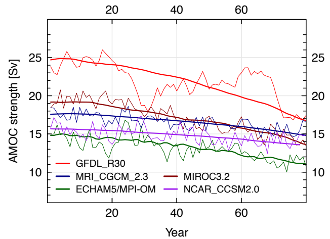
Fig. 3. Comparison of the calibrated model outcome (thick line) with the AOGCM reference data for the 1 % \text{CO}_2 increase scenario from Gregory et al. (2005) (thin line). Our emulation outcome reproduces the weakening trend of all five AOGCMs.
