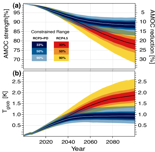
Fig. 4. Probabilistic future projections for the RCP3-PD and RCP4.5 scenario relative to the year 2000: (a) AMOC based on the equally weighted five model ensemble (individual model projections are shown in Fig. S1 of the Supplement). (b) Corresponding global mean temperature obtained from the MAGICC6 model emulating IPCC AR-4 models.
