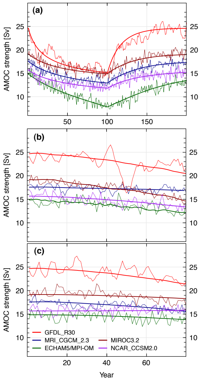
Fig. 2. The results of the calibration procedure, the thin line represents the AOGCM output, the thick line the best fit results of our emulation. (a) The freshwater hosing experiment by Stouffer et al. (2006), where 0.1 Sv are artificial added in the Northern North Atlantic for 100 years starting in year 1. (b) The transient change in the AMOC strength as presented in Gregory et al. (2005) for a scenario with a compounded 1 % per year increase in the \text{CO}_2 concentration, while the freshwater fluxes are kept constant. (c) The same scenario as in (b) , but with constant \text{CO}_2 -concentrations, whereas the freshwater fluxes of the full transient scenario are applied.
