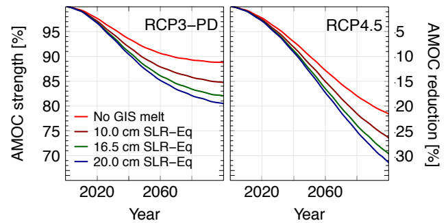
Fig. 5. Projections of the probabilistic ensemble median AMOC-reduction for different Greenland meltwater influx scenarios for the RCP3-PD (left panel) and the RCP4.5 (right panel) emission pathway. Additional freshwater forcings correspond to 10, 16.5 and 20 cm Greenland contribution to global SLR by 2100.
