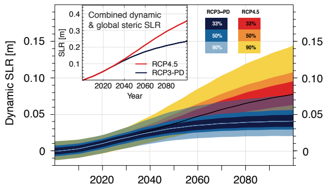
Fig. 6. Probabilistic projections of the mean dynamic sea-level rise at the New York City coastline for the RCP3-PD (blue) and the RCP4.5 (orange) emission pathway until 2100. We project a median dynamic sea-level rise of 4 cm for the RCP3-PD and 8 cm for the RCP4.5 scenario. Inlay: Estimates of the steric and dynamic sea-level rise at the New York City coastline by combining our projections with simulations of the global steric sea-level rise by Schewe et al. (2011).
