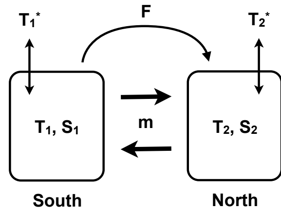
Fig. 1. Schematic view of our conceptual two box model for the Atlantic Meridional Overturning Circulation.
