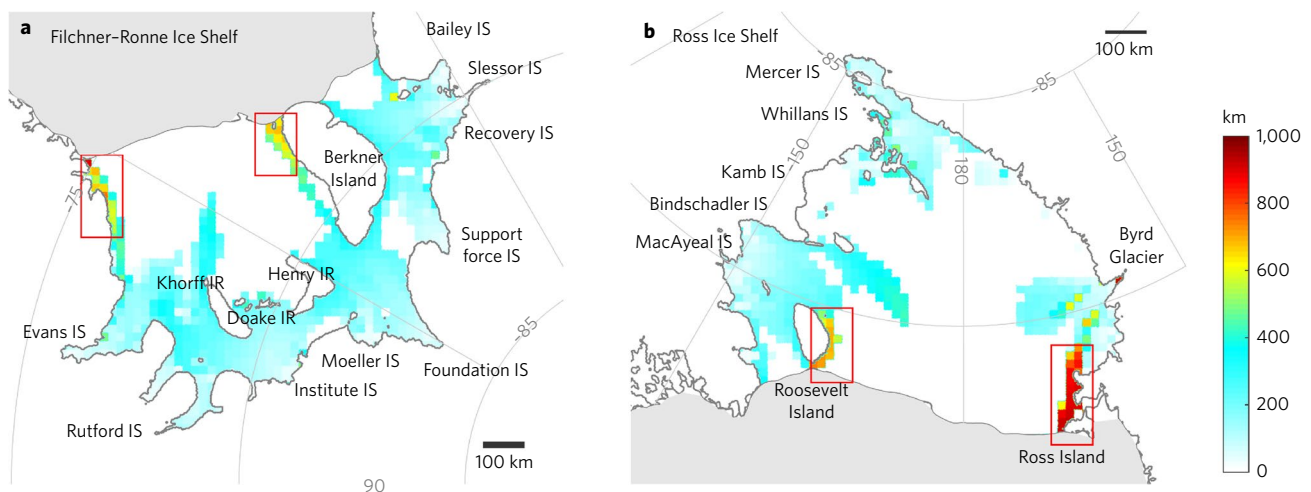
Fig. 3 | Tele-buttressing. a, b. The maximal response distance for every perturbation location of Filchner-Ronne (a) and Ross (b) Ice Shelf. The maximal response distance is defined as the maximum distance for which the remote buttressing flux response number, that is, the response ratio over all grounding lines that are farther away than this distance, is greater than a threshold of 0.02%. Ocean is shown in grey.
