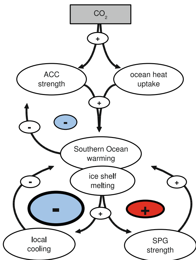
Fig. 10 Rising atmospheric temperatures (CO 2 ) enhance SO warming and associated ISM in two ways. Isopycnal diffusion transports heat to depth and increases the meridional temperature gradient across the ACC (ocean heat uptake). In addition to increased southward mixing of heat, the accelerated ACC enhances southward advection of heat (ACC strength). Initially, steepening of isopycnals is dampened by less northward export of sea-ice, until its decline saturates (not shown). If basal melt fluxes are coupled to the ocean, ISM will be weaker. Mixing limited local cooling at the shelves forms a dominating negative feedback. Secondly, the gyres reveal a self-amplifying feedback with ISM. Melted freshwater increases the across gyre density gradient (SPG strength), causing an additional warming of the SO. As a minor negative feedback, ISM also dampens the increase of ACC strength
