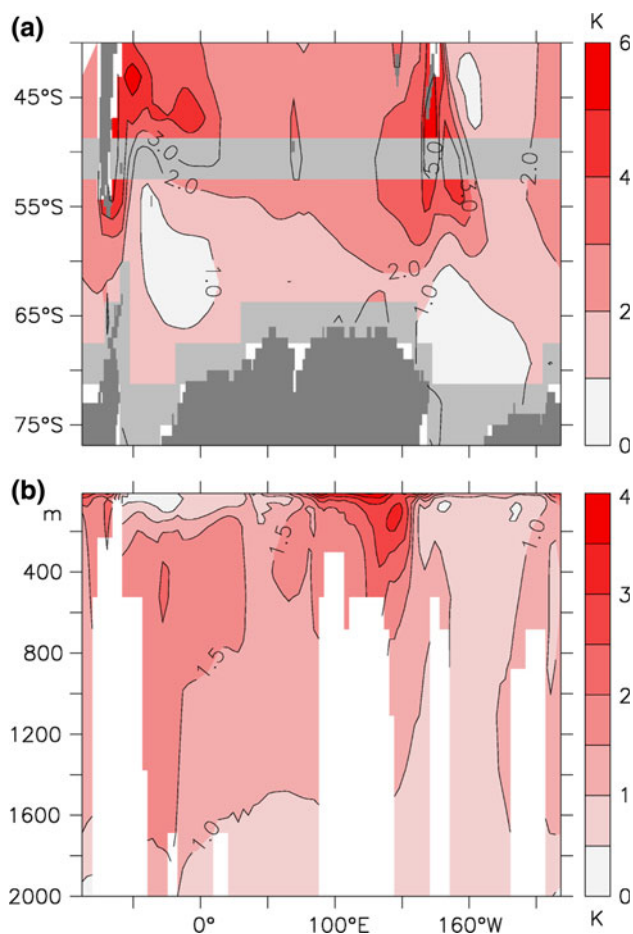
Fig. 6 a Mean temperature anomaly in the SO averaged to 2,000 m depth after 200 years in the noISM run. b Cross-section of meridional mean temperature anomaly after 200 years in the shaded area in a framing the Antarctic continent. SO warming is strongest below the surface and coincides with large-scale advection patterns. Areas shaded in grey also indicate areas where potential energy is determined in Sect. 3
