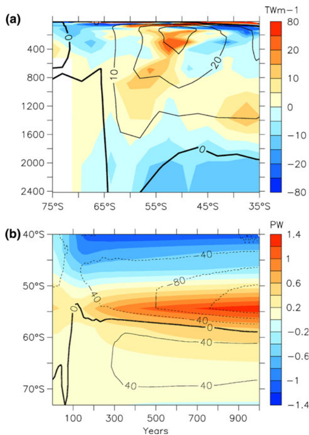
Fig. 7 a Zonal mean southward heat transport anomaly from advection and eddy diffusion after 1,000 years (noISM run). Contours indicate the Deacon cell (Sv). Advection warms the SO below the surface. b Hofmueller diagram of southward advective heat transport in the noISM run (colors) and additional anomaly due to ISM with = 1 (TW, contours). The total southward advection of heat is well correlated with ACC strength. ISM causes additional heat transport in the enhanced SPGs
