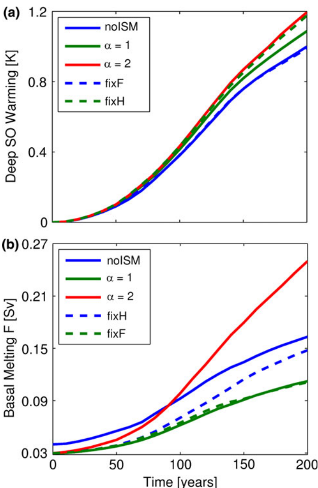
Fig. 8 Timeseries of a SO mean temperature anomaly between 500 and 2,000 m depth south of 62° for different experiments b Timeseries of total ISM fresh water flux in different experiments. Basal melting increases as the deep ocean temperature increases and enhances heat transport towards the SO
