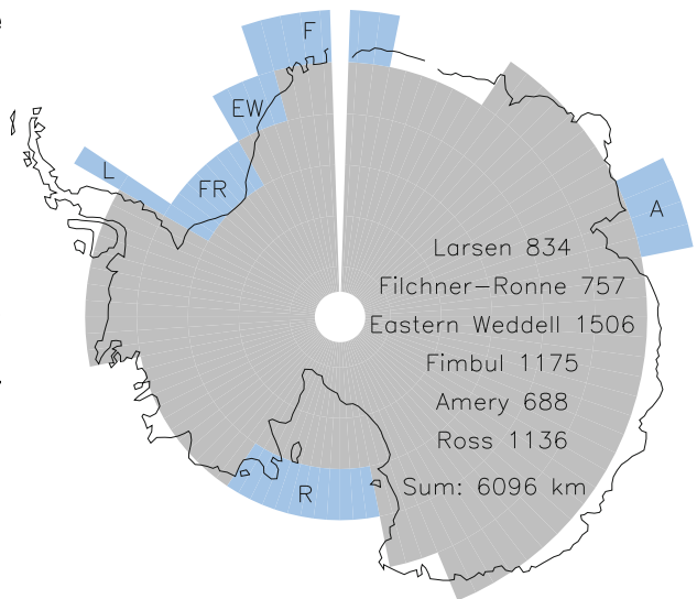
Fig. 1 Representation of individual ice shelves in CLIMBER-3 \alpha geometry, framing the ocean model boundary (coastline in the model covered by ice shelves). Length of coastline in the model covered by ice shelves (staggered grid). Ocean mean temperatures are diagnosed between 200 and 600 m depth and compared with the freezing point of sea water at 200 m depth. Sub-surface heat and fresh water fluxes are injected at the same place
