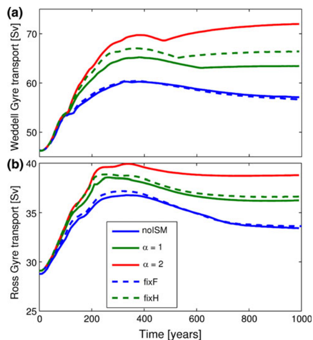
Fig. 5 Timeseries of Weddell Gyre and Ross Gyre transport for different experiments. ISM increases gyre strength under global warming
