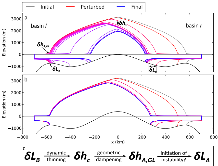
Figure 4. Profiles of the transient ice sheet between the end of perturbation (red) and the final steady-state (blue) for two different values of central bed elevation (a) b_c = 0 m (example of unstable scenario U, same as in Fig. 3a) and (b) b_c = +400 m (example of stable scenario S). The time interval between two consecutive profiles is 1 kyr. The bottom panel explains the mechanism of basin interaction conceptually with the notation depicted in panel (a) .
