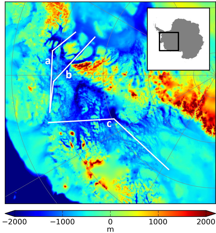
Figure 1. Topographic map of the bedrock underlying the Antarctic Ice Sheet. Each of the transects (white lines) connects two major drainage basins of the WAIS. The bed topography and the ice profile along transects a, b and c are shown in the corresponding panels of Fig. 2.
