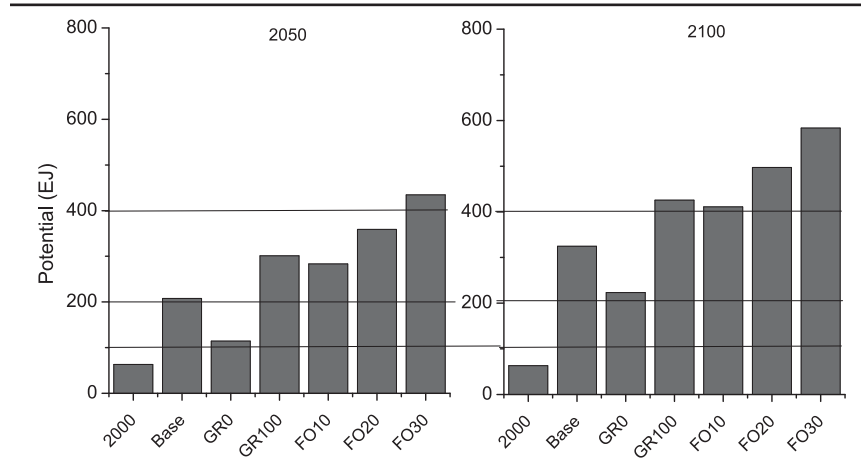
Figure 5. Impact of Using Natural Areas on Woody Bio-Energy Potential
