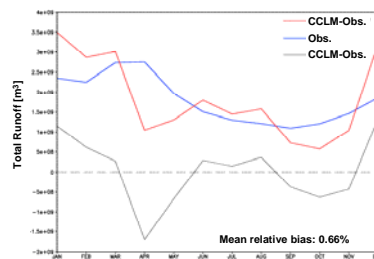
Climatological monthly cycle runoff, Elbe river catchment, 1970-1999
