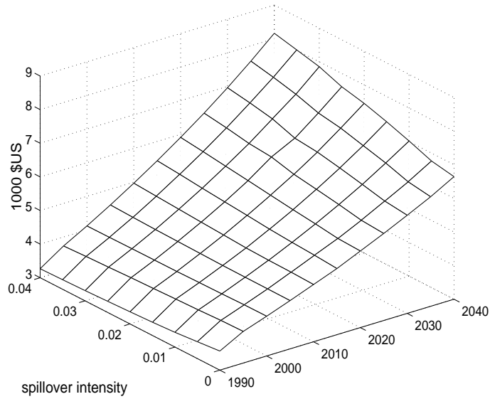
Figure 9: Per capita consumption sensitivity on spillover intensity in IR (developed world region)
