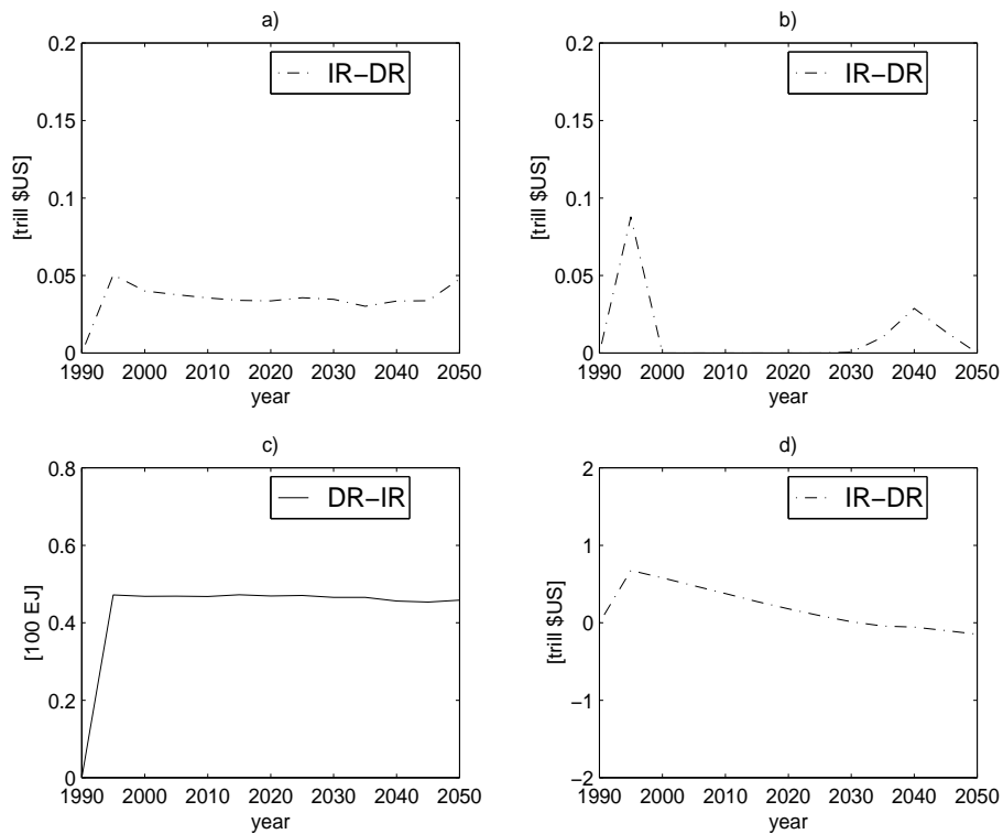
Figure 4: Net export of a) consumption goods, b) investment goods, c) primary energy (first mentioned region in the legend always denotes the exporter), and d) net foreign assets - discounted (IR - developed world region, DR - developing world region).
