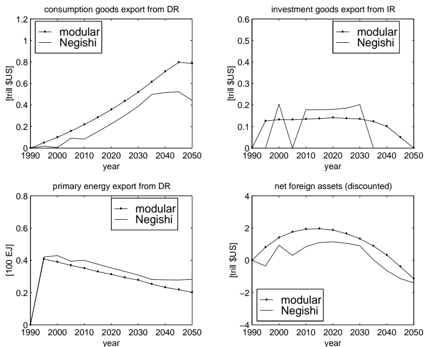
Figure 7: Trade structure and net foreign assets in the spillover case.
