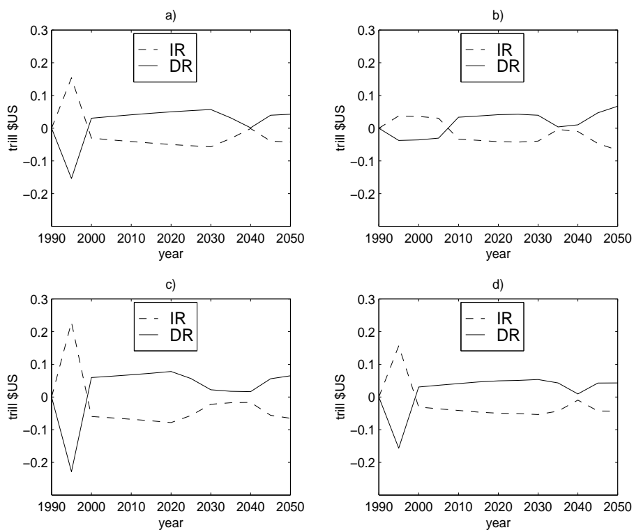
Figure 3: Current account resulting from the Negishi approach (a) and from the modular approach after (b) 10 iterations, (c) 40 iterations, (d) 300 iterations (IR - developed world region, DR - developing world region).
