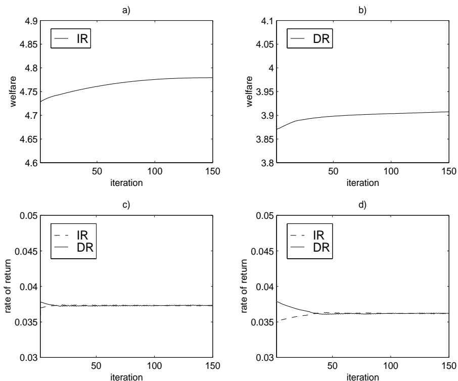
Figure 2: Convergence of welfare (a and b) and return rates on capital in 2015 (c and d) (IR - developed world region, DR - developing world region).
