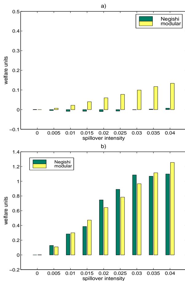
Figure 5: Welfare difference between spillover and non-spillover cases in a) IR (developed world region) and b) DR (developing world region).
