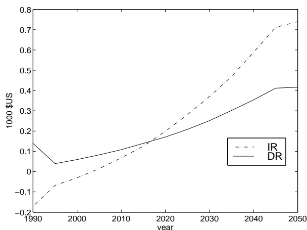
Figure 6: Per capita consumption gains from spillover effects (IR - developed world region, DR - developing world region).
