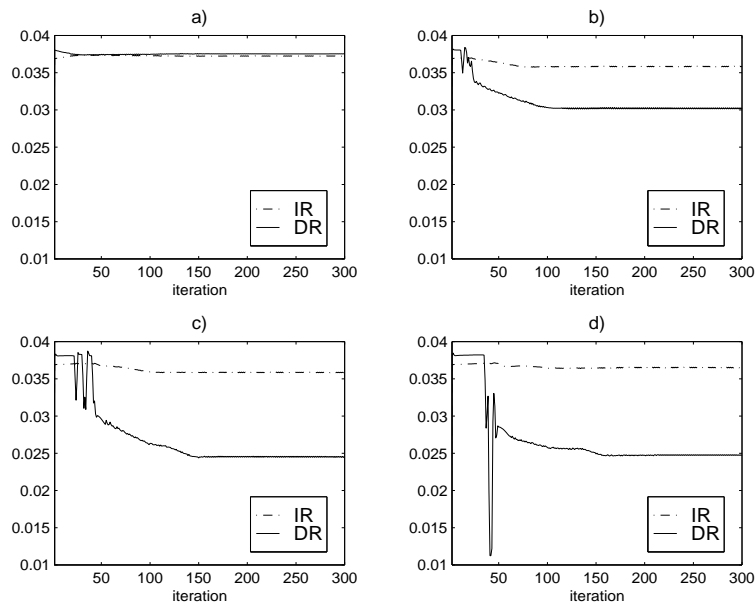
Figure 10: Convergence of return rates in 2010 with varying spillover intensity: a) \beta=0.0 , b) \beta=0.02 , c) \beta=0.04 , d) \beta=0.06 (IR - developed world region, DR - developing world region).
