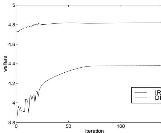
Figure 8: Convergence of welfare measure (IR - developed world region, DR - developing world region).
