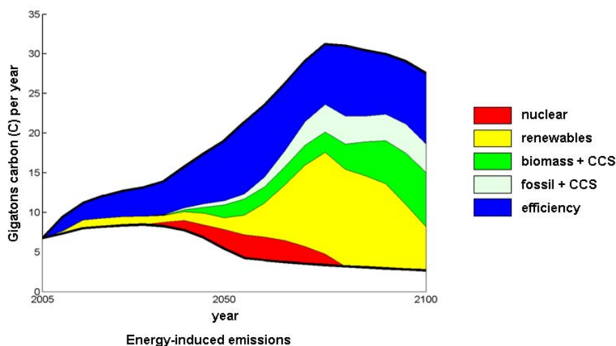
Figure 2: Contribution of mitigation options to global emission reductions in the energy sector for a scenario with cheap fossil fuels. Source: REMIND-G.
