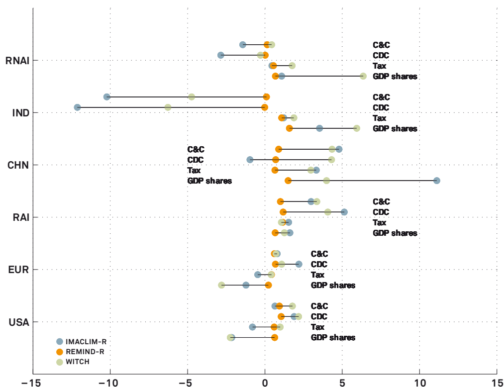
FIGURE 2-8 Distributional effects of various allocation schemes to achieve 450 ppm CO 2 only in terms of consumption losses for the models IMACLIM-R (blue), REMIND-R (orange) and WITCH (green). Percentage changes are given relative to baseline using a 3% discount rate. The figure shows the ranges of consumption losses over the different models and regions which can be interpreted as uncertainty ranges
