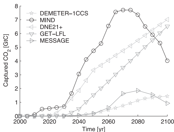
Figure 12. Carbon Capture and Sequestration Over the Course of the Century
