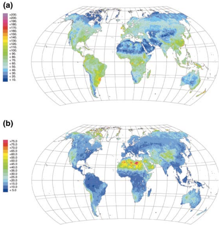
Fig. 2 Spatial distribution of the variability in NPP estimates among the models as represented by (a) the standard deviation of model NPP estimates in a grid cell; and (b) the coefficient of variance of model NPP estimated in a grid cell. The coefficient of variance is determined by dividing the standard deviation by the mean of the model NPP estimates within a grid cell.
