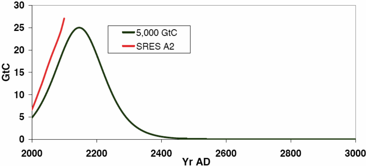
Figure 2: Feasible emissions with available carbon (Archer and Brovkin, submitted), black. IPCC SRES A2 fossil fuel emissions for 21st century, red.
