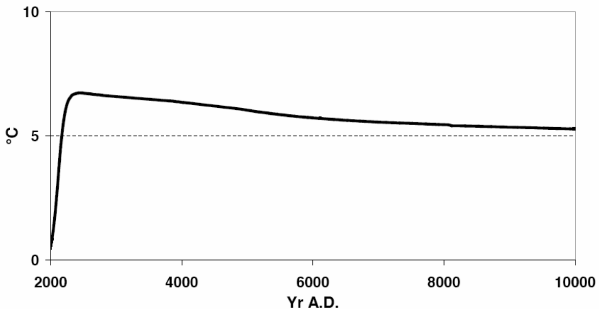
Figure 3: Temperatures resulting from the emissions of Figure 2 (Archer and Brovkin, submitted).
