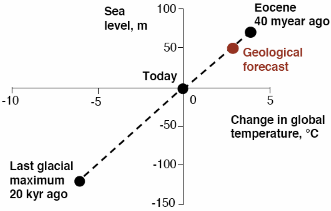
Figure 4: The relationship between sea level and temperature on geological timescale. Modified from Archer (2006, Fig. 12.7).
