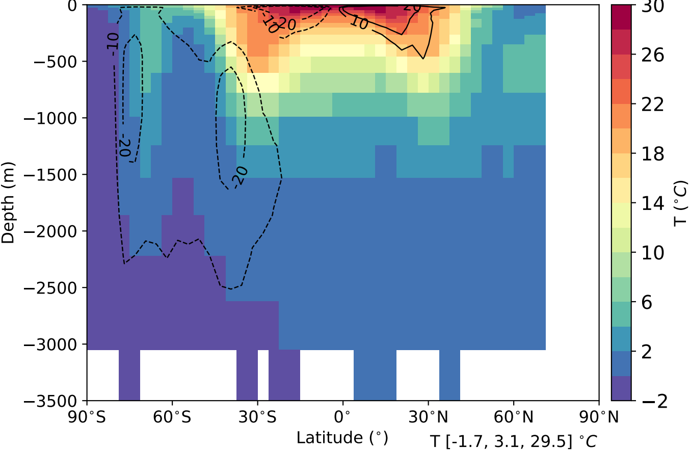
Temperature (at 180°W) & Global Overturning Streamfunction ( S_v )
