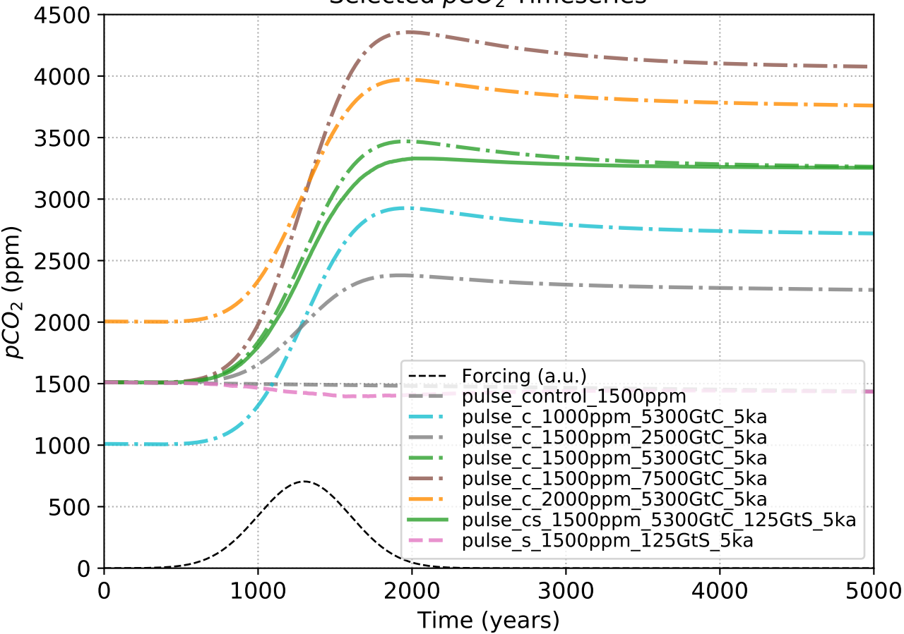
Selected p\text{CO}_2 Timeseries
